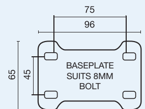
Baseplate for 75-125mm Rigid Castors
