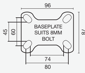
Baseplate for Rigid Castors
