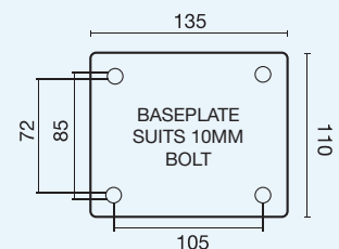
Baseplate for 150-200mm Swivel Castors
