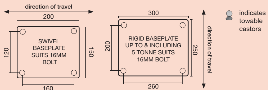
Standard baseplate dimensions & drilling patterns for Twin Wheel EHP castors
