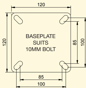
Baseplate for Richmond Floor Locks
