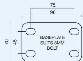
Baseplate for 75-125mm Swivel Castors
