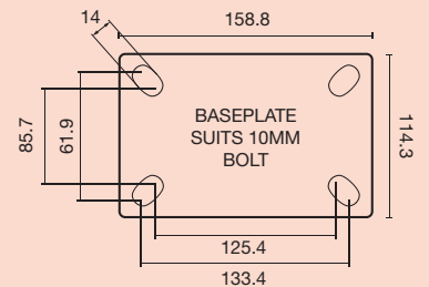
Baseplate dimensions & drilling patterns for Shock-Absorbing castors
